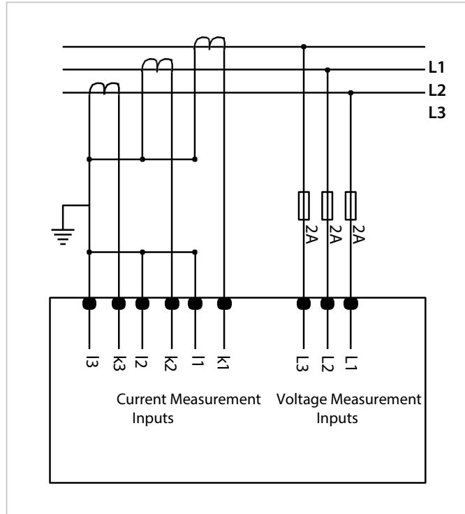
Fig. 2-7 KLEA 3 Phase Delta Connection Diagram
