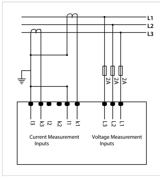
Fig. 2-8 KLEA Aron Connection Diagram
