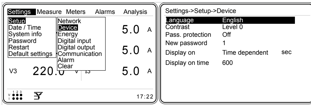
Fig. 3-19 Device Menu
