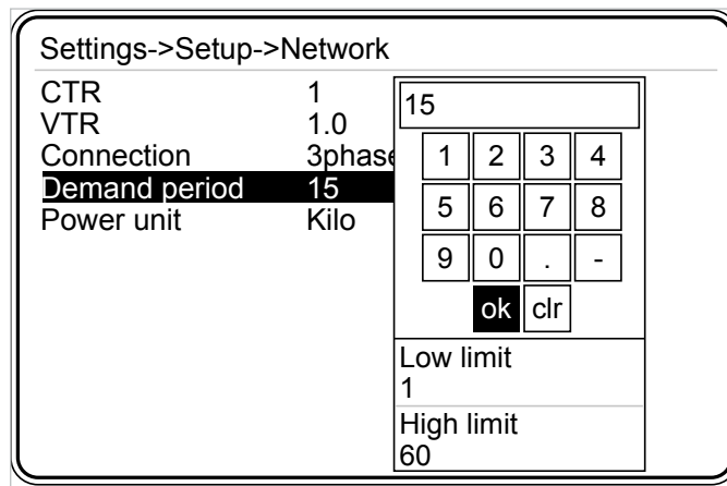
Fig. 3-17 Demand Period
