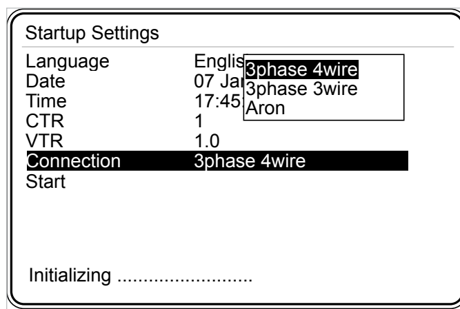
Fig. 3-8 Connection Types
