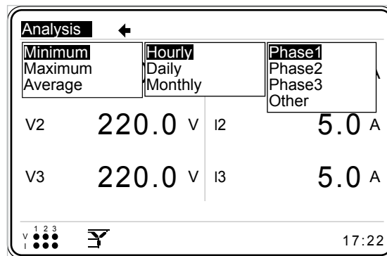
Fig. 3-92 Hourly Menu
